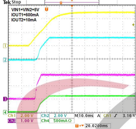
Power ON Test (Channel1)
